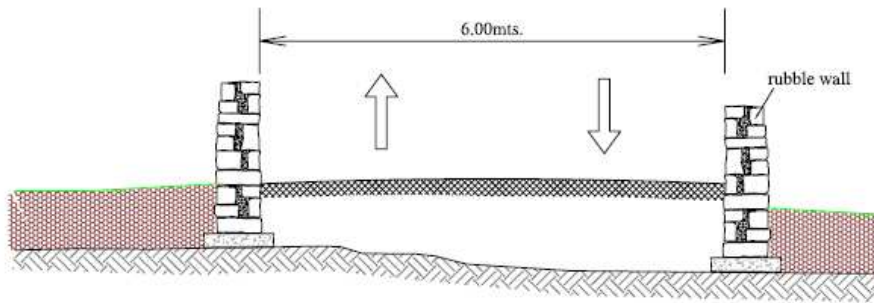
Proposed Section AA
