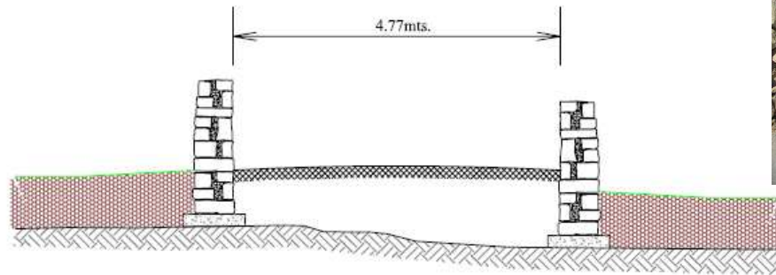
Existing Section AA
