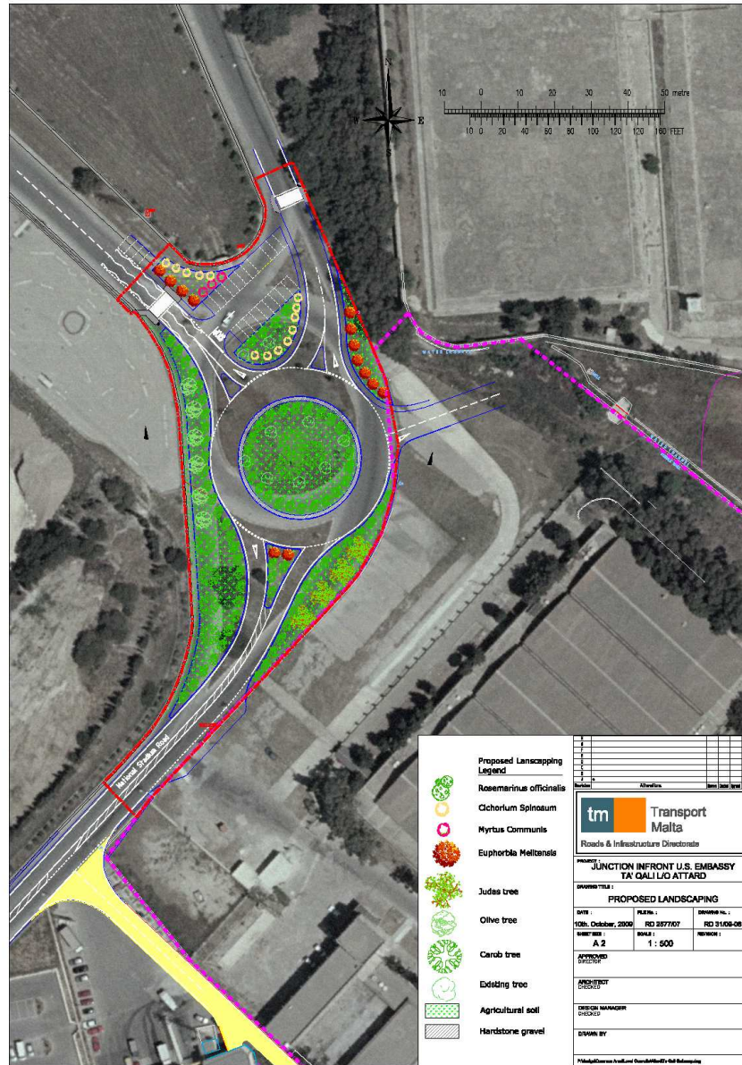
Proposed Junction
